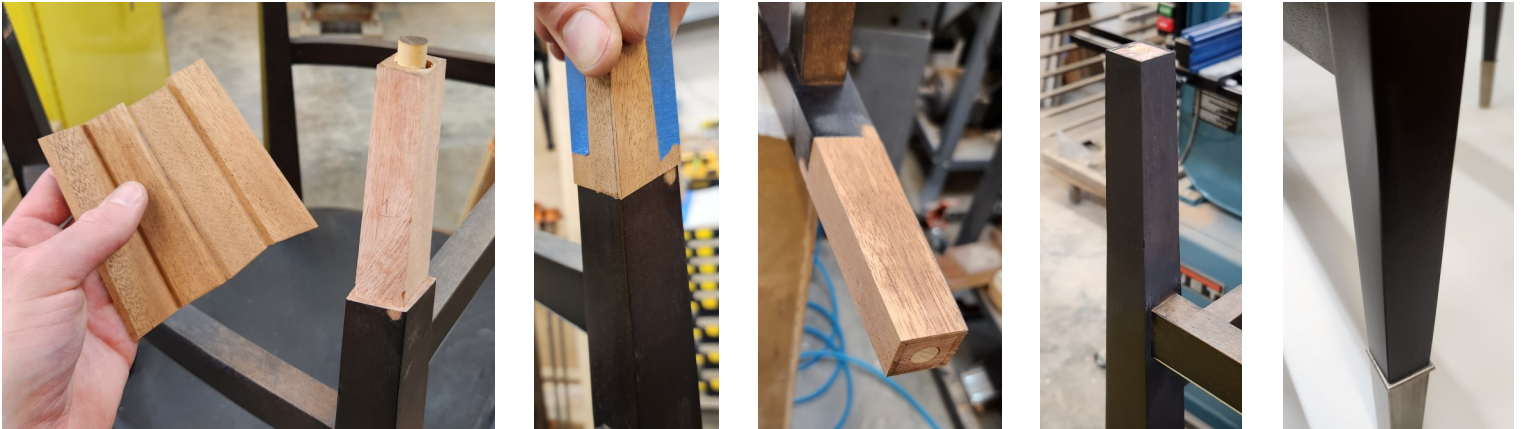
Tapered chair leg with miter-folded patch; stained and finished to match.
